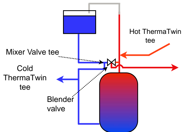
Correct Mixer Valve Installation
